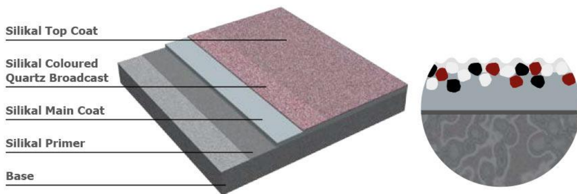
Figure 1: Composition Kitchenfloor
